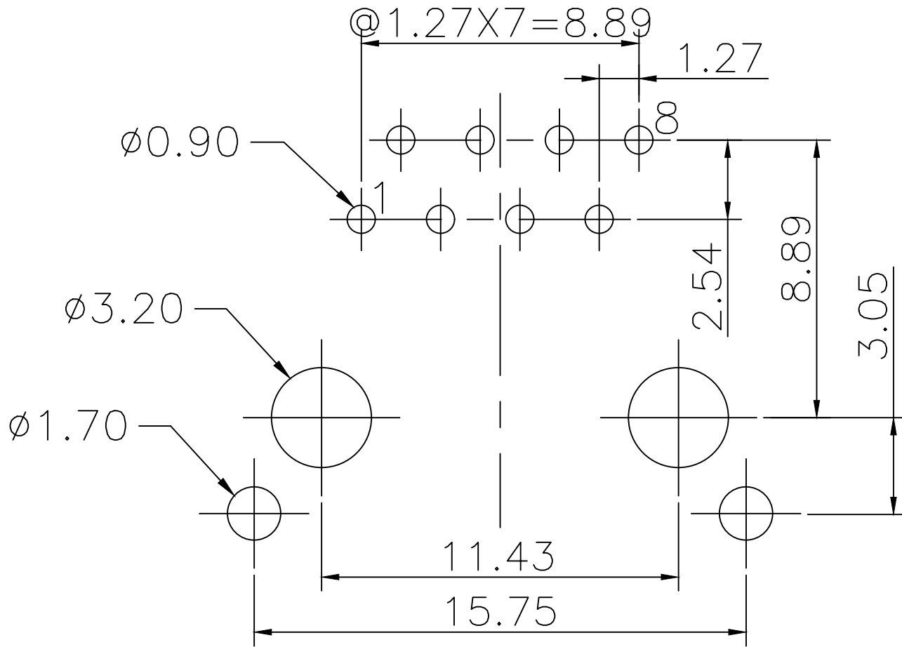
PC Board Layout Component Side Shown
